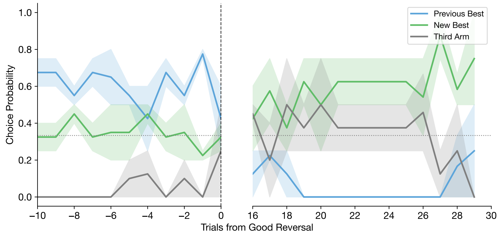
Good Reversal-Aligned Choices (mean \pm se across subjects | n=2 subjects, n=9 reversals) (Skipping first 15 trials post-reversal)
